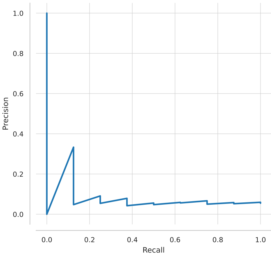
Precision-Recall Curve - RF
